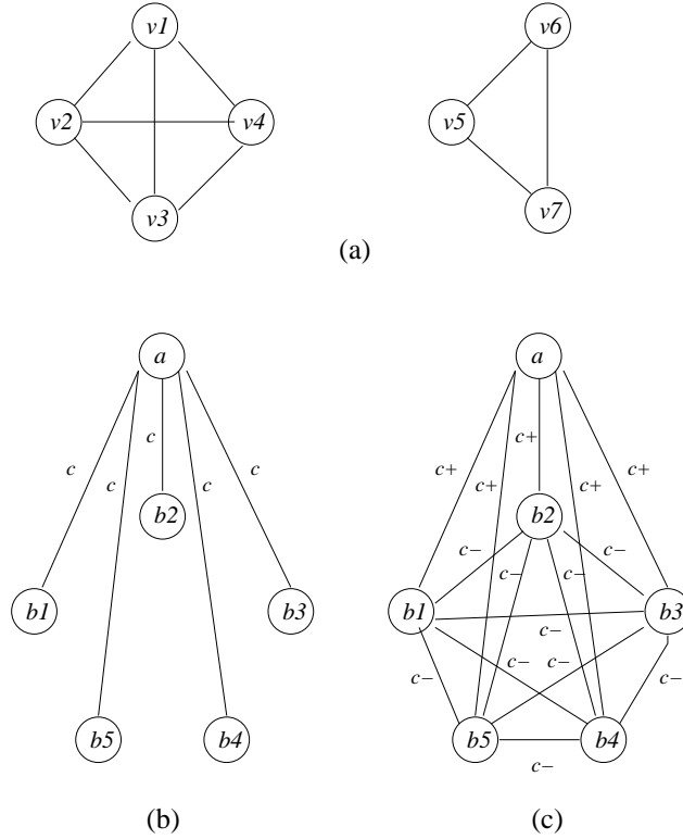
Fig. 1. Near-Optimal Solution Value Does Not Imply Near-Optimal Solution Structure. (a) Graph G_3 . (b) Graph X_5 . (c) Graph Y_5 . See main text for details.
