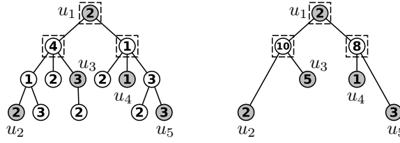
■ Figure 2 Left : An example tree. The highlighted nodes constitute set U of Definition 8. Set L of Definition 8 consists of the nodes within boxes. Note that the root node u_1 is by definition in B , however, it is also in L since \text{lca}_t(u_3, u_4) = u_1 . Right : The structure tree ST(U) .
