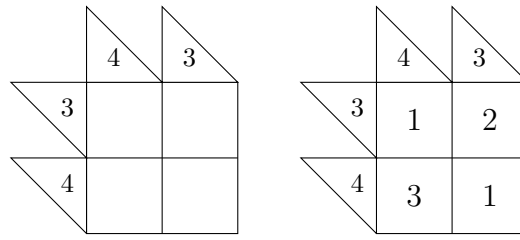
■ Figure 4 Simple example of a Kakuro grid and its solution.
