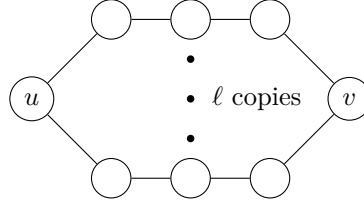
■ Figure 1 The gadget H_\ell of Provan and Ball [16] as used in the proof of Theorem 3. It corresponds to an \ell -fattening of the edge \{u, v\} , followed by a 4-stretch of each of the \ell parallel edges.
