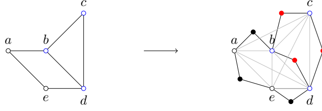
■ Figure 2 Example of the construction in Theorem 6.1. The left-hand side shows the original graph, the right-hand side the graph constructed by the reduction, where the newly introduced edges between each pair of vertices of the original graph are drawn in grey. The vertices introduced for each edge of the original graph are filled red and black, the corresponding new edges are drawn in black. Note that the blue vertices of the original graph form a clique and that the vertices corresponding to the edges of said clique (filled red) form an independent set in the new graph.
