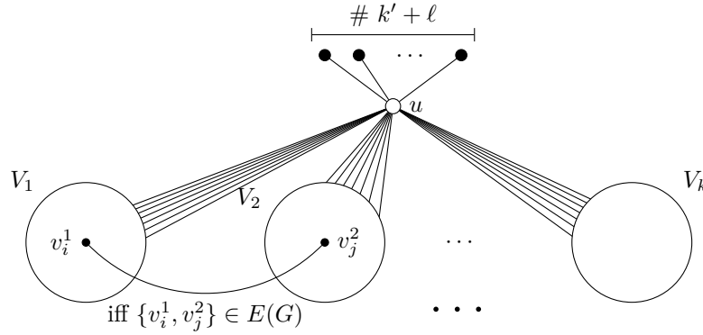
■ Figure 1 Sketch of the construction in proof of Theorem 5.4. The circles refer to cliques with vertex set V_i , i \in \{1, \dots, k\} .
