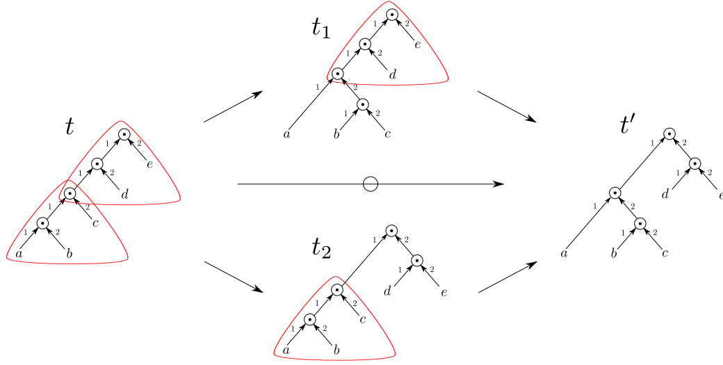
Figure 1 The application of a multi-step t \twoheadrightarrow t' where t = (((a \cdot b) \cdot c) \cdot d) \cdot e and t' = (a \cdot (b \cdot c)) \cdot (d \cdot e) . This multi-step t \twoheadrightarrow t' intuitively corresponds to the simultaneous application of two instances of the associativity rule (x \cdot y) \cdot z \rightarrow x \cdot (y \cdot z) to t . The regions surrounded by red curves indicate the portions of the term identifying a match for the left-hand side of the rule. The multistep can be decomposed in two ways as a sequence of individual rewriting rules: either as t \rightarrow_{\mathfrak{R}} t_1 \rightarrow_{\mathfrak{R}} t' or as t \rightarrow_{\mathfrak{R}} t_2 \rightarrow_{\mathfrak{R}} t' .
