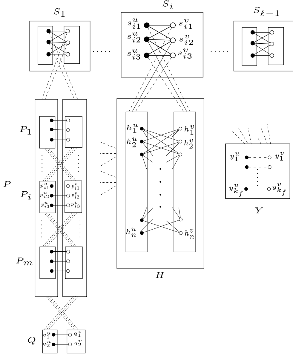
Figure 1 Illustration of the construction of G . The black nodes denote the vertices in U(G) , and the white nodes denote the vertices in V(G) . The solid edges represent edges in E^{imp} , and the dashed edges denote edges in E^{free} . The edges between P and H and those between Y and G \setminus Y are not shown. The edges shown between S_i and H are present for all i \in [\ell - 1] , whereas the edges shown between S_1 and P are only present for S_1 and not for any S_i for i \geq 2 .
