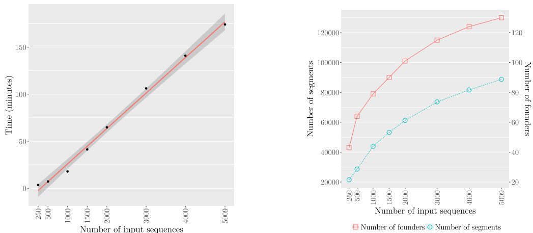
(a) The running time of our implementation plotted against the number of input sequences with L = 10 . The data points have been fitted with a least-squares linear model, and the grey band shows the 95% confidence interval.
