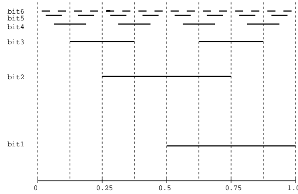
Fig. 1. Gray code Embedding of real numbers.
