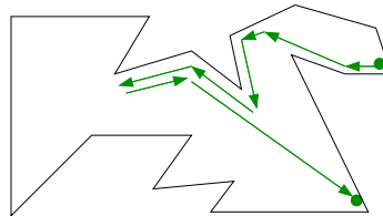
Fig. 15. Computed solution paths for catching the evaders in the given environments.
