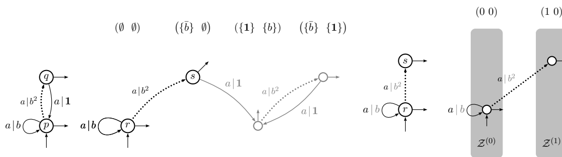
(a) A lag separation covering \mathcal{U}_N with N = 1 . The \mathfrak{P}(\Delta_1)^Q -vectors (vertical projection) are indexed by \{p, q\} , in that order. The dotted transition is larger than the solid one. The input-2-ambiguous (and equivalent to \mathcal{T} ) subtransducer \mathcal{V}_1 is reduced to the states \{r, s\} .
