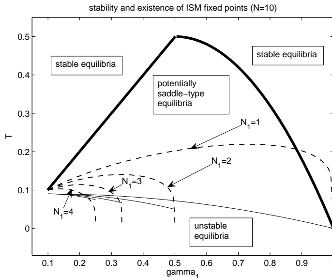
Figure 3: Stability regions for equilibria \mathbf{w} \neq \bar{\mathbf{w}} of ISM with N = 10 units as a function of the larger coordinate \gamma_1 and temperature T . The number of coordinates with value \gamma_1 is denoted by N_1 . Temperatures T_s(\gamma_1) (30) above which equilibria with larger coordinate equal to \gamma_1 are guaranteed to be stable are shown with solid bold line. For N_1 = N - \ell \in \{1, 2, 3, 4\} , we show the temperatures T_u(\gamma_1; N, \ell) (32) below which equilibria with larger coordinate equal to \gamma_1 are guaranteed to be unstable with solid normal lines. Also plotted are temperatures T_e(\gamma_1; N, \ell) (9) at which equilibria with the given number N_1 of coordinates of value \gamma_1 exist (dashed lines).
