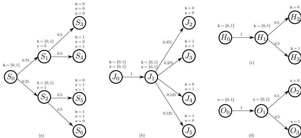
Figure 3 Bit XOR example: a) Markov chain semantics \mathcal{C} . b) Joint marginal \mathcal{C}_{|(o,h)} . c) Secret's marginal \mathcal{C}_{|h} . d) Observer's marginal \mathcal{C}_{|o} .
