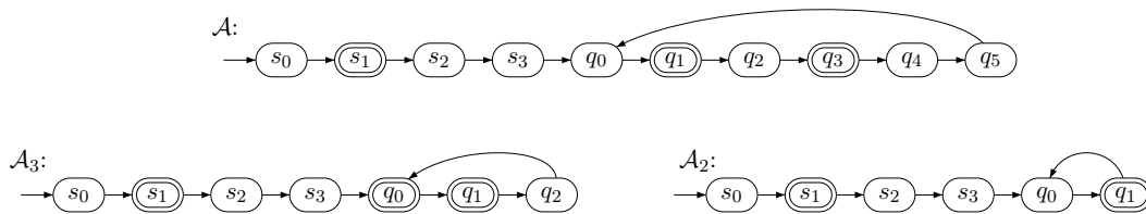
■ Figure 2 The DFA \mathcal{A} and its clean quotients \mathcal{A}_3 and \mathcal{A}_2 .
