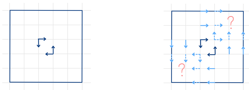
(a) A monotone function f : [6]^2 \rightarrow [6]^2 with f(3, 4) = (4, 3) and f(4, 3) = (3, 4) . (b) The standard partial information derived by (3, 4) and (4, 3) , described in the light blue color. The solid arrows mean -1 or 1 and the dashed arrows mean \leq or \geq (the same rule applies below).
