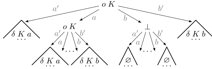
■ Figure 3 Trie for deferred concatenation L \hat{\ } K .
