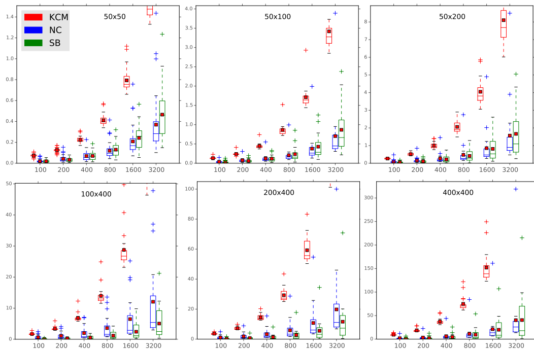
■ Figure 2 Boxplots of running times in seconds for grid graphs. Plus signs represent outliers. A red square marks the mean. The x-axis corresponds to different values of k and uses a logarithmic scale.
