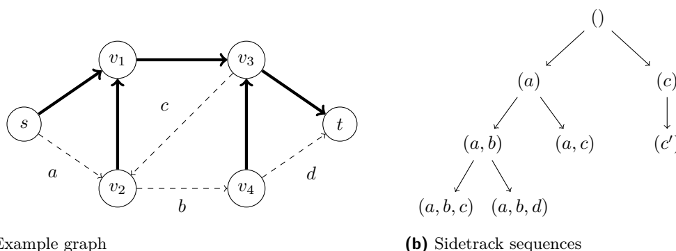
Figure 1 Example for the basic algorithm. In Figure 1a, the thick, solid edges belong to T_0 . In Figure 1b, every sidetrack is associated with T_0 except for c' , which is associated with the SP tree T_1 comprising the edges b and d . An arrow from sequence p to sequence p' indicates that p is the parent path of p' .
