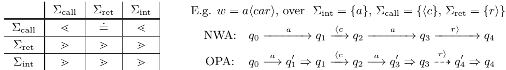
■ Figure 5 The OPM M for VPL and an example of the translation of runs from NWA to OPA.
