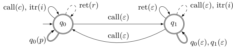
■ Figure 4 The wOPA \mathcal{A}_{\text{log}} nondeterministically writes logs at different levels of detail.
