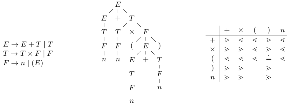
■ Figure 1 A grammar generating arithmetic expressions (left), an example derivation tree (center), and the precedence matrix (right). E.g. M[1, 2] = < means that + yields precedence to \times .
