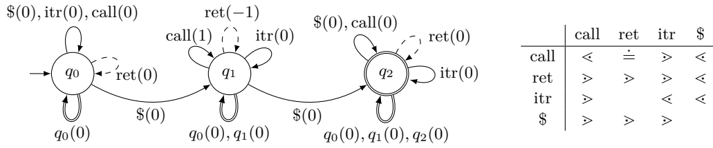
■ Figure 3 The weighted OPA \mathcal{A}_{itr} penalizing unmatched calls nondeterministically, and its precedence matrix (right). Weights are given in parentheses at transitions. The weight semiring is \mathbb{Z}_{\max} = (\mathbb{Z} \cup \{-\infty\}, \max, +, -\infty, 0) .
