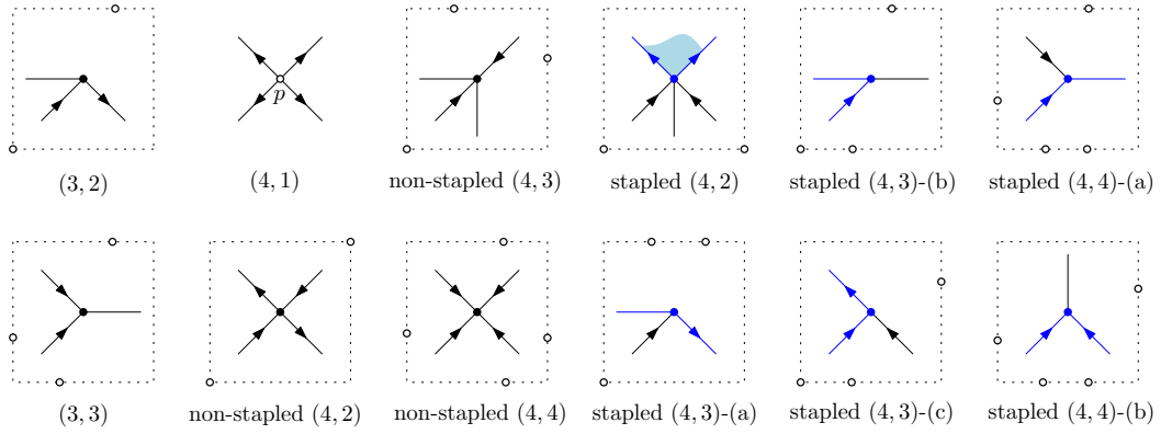
■ Figure 3 Illustration of the 12 vertex types of VD(\theta) labeled with their type names. Dotted squares and small circles on them depict an empty square corresponding to each vertex type and its contact points. Dots and line segments depict vertices and all incident edges to each vertex; in black if regular, or in blue, otherwise. The arrows on edges depict the direction in which the corresponding square grows. The shaded area in the stapled (4, 2)-type depicts a neutral face which does not belong to any Voronoi region VR_p(\theta) for p \in P . (We keep the above convention on every figure in this paper.) Note that the right six types are stapled, while the left six are not.
