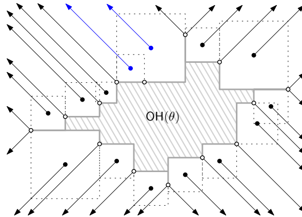
■ Figure 4 Illustration to Lemma 3.3. The orthogonal convex hull \text{OH}(\theta) of P (shaded region) and the four staircases (gray thick lines) describe all unbounded edges (arrows) and their incident vertices of \text{VD}(\theta) (small circles and dots).
