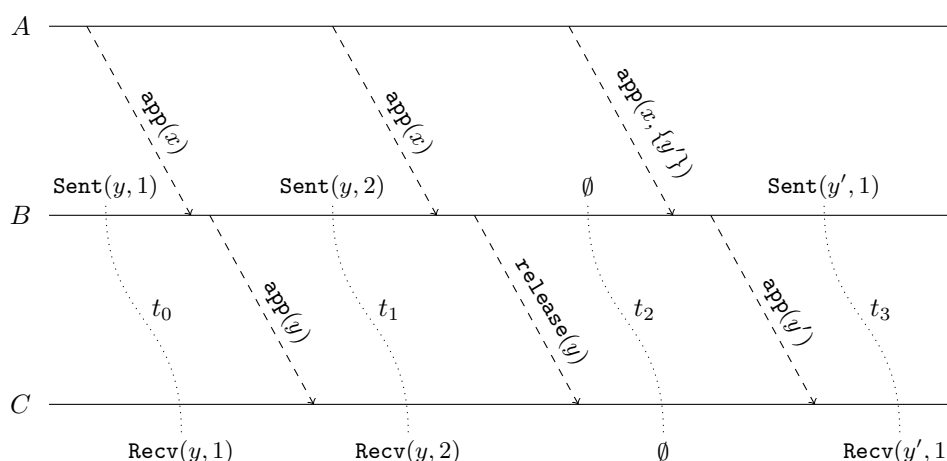
■ Figure 3 A time diagram for actors A, B, C , demonstrating message counts and consistent snapshots. Dashed arrows represent messages and dotted lines represent consistent cuts. In each cut above, B 's message send count agrees with C 's message receive count.
