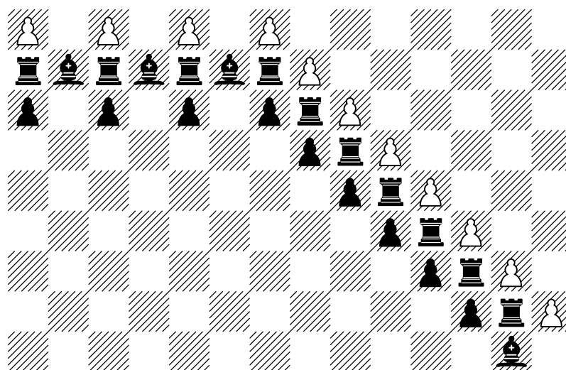
■ Figure 9 Terminator gadget that connects the loose ends of gadgets to the bottom rank. Unlike other figures, here we care that the first rank of this figure is the actual first rank of the Chess board. In particular, this means that the white pawn on the second rank cannot unmove, and that allows us to prove that everything is stuck.
