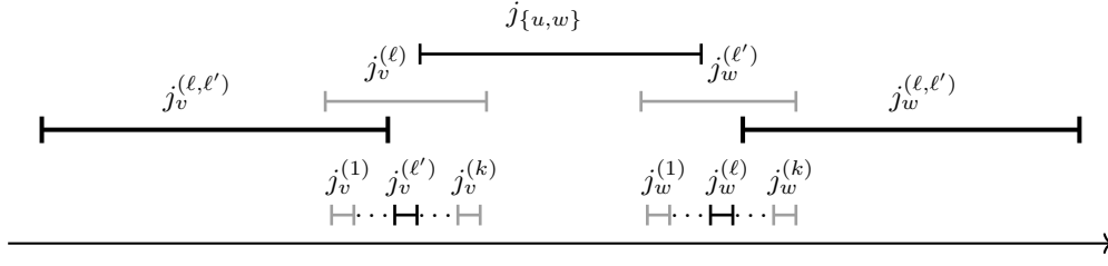
■ Figure 1 Illustration of the edge selection machine for color combination \ell, \ell' with \ell < \ell' . Depicted are intervals of jobs relating to v \in V_\ell , w \in V_{\ell'} , and e = \{v, w\} \in E . Gray intervals correspond to jobs that are not eligible on the machine.
