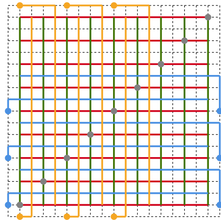
(b) Reserved wires on layers 1 through 4, including all possible I/Os, for template in theorem 17. Locations of I/Os and gate variables are indicated.
