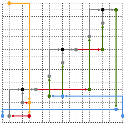
(c) Layout for example circuit as produced by the construction in theorem 17. Inputs at north 0 (the 0-th point on the north boundary) and east 0; output at west 0. Gates and nodes with between-layer connections are indicated.
