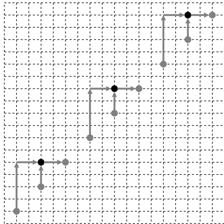
(a) Three 2-input, 1-output gates implemented on the diagonal on layer 0 as in theorem 17. Black nodes indicate where the gate itself is placed.
