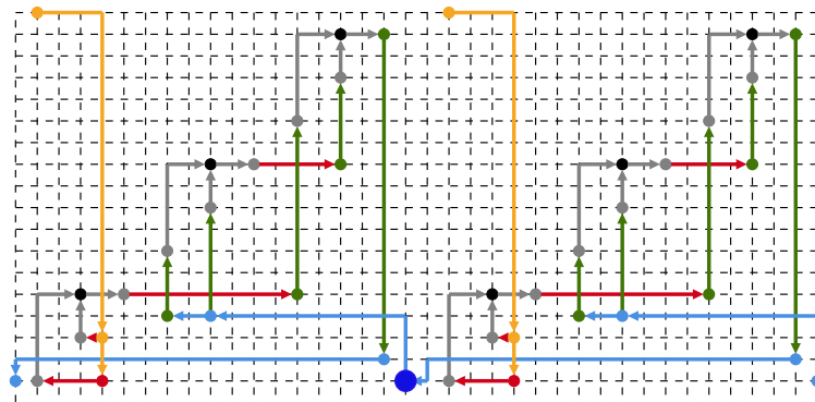
(e) Two example circuits placed next to each other and connected output-to-input as in Theorem 18. The large dark blue node indicates where a flip-flop is placed.
