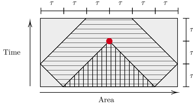
■ Figure 3 Side view of 6\tau \times 6\tau \times 3\tau volume for the serialization case of Lemma 22. The red point is where C[j] is produced; vertical lines indicate the volume where inputs A[i] may be read, and horizontal lines indicate the volume where outputs C[i] may be produced, for i \in S' .
