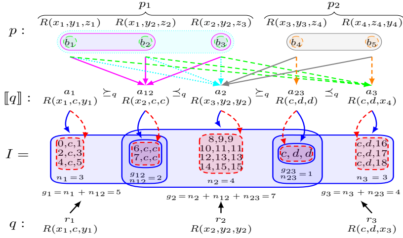
■ Figure 1 A three-atom JoFBQ q , the associated minimal unification closure \llbracket q \rrbracket with homomorphic ordering \preceq_q among its five atoms a_i , a multicanonical instance I for q , and a BCQ p obtained as the cross-product of the two BCQs p_1 and p_2 .
