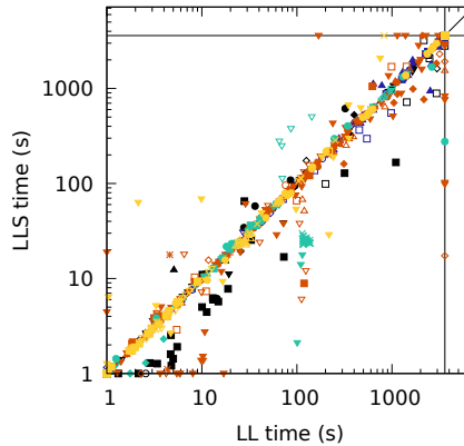
■ Figure 5 Runtime Comparison: LL vs. LLS.
