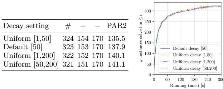
■ Figure 13 Effects of diversifying Kissat’s decay parameter.
