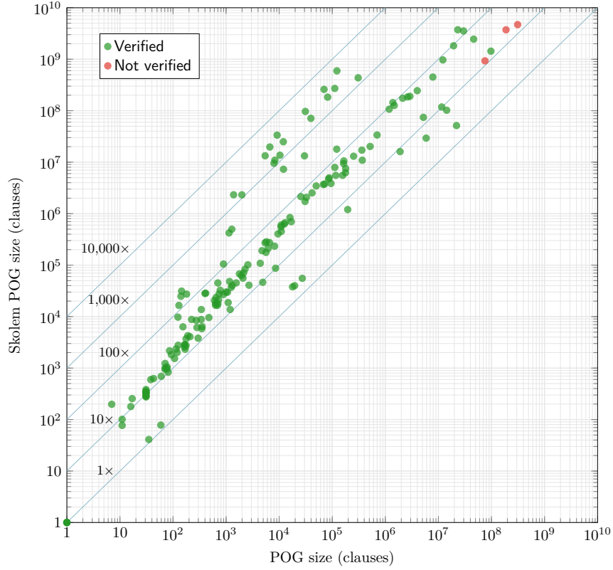
■ Figure 6 Skolem POG overhead. Skolem POG size vs. POG size. The median size ratio was 34 \times . Colors indicate the level of success achieved in verification.
