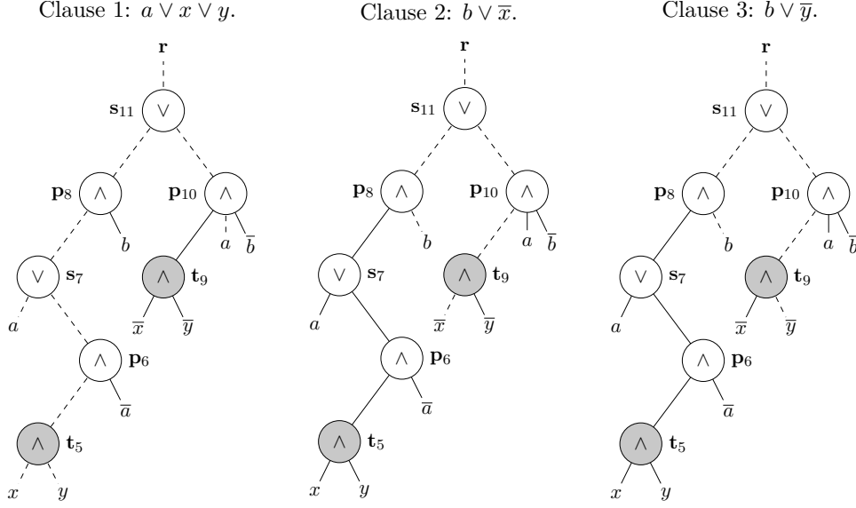
■ Figure 3 Justifying input clause deletions. Negating the clause literals and then unit propagating through the operations cause the Skolem POG to evaluate to 0. Literals assigned value 0 are shown as dashed lines.
