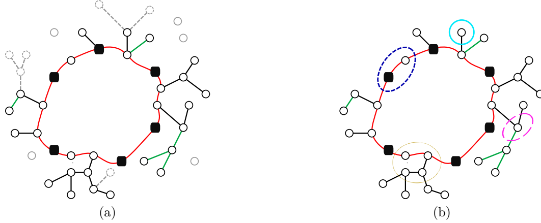
■ Figure 1 (a) The graph T'' after pruning and picking up critical vertices. The terminals in O are drawn as black rectangles. The cycle C is depicted in red, the surviving edges of R are drawn in black and edges in F_P in green. The greyed out vertices and edges do not belong to T'' . They have either been pruned (the dashed vertices and edges), not sampled, or split off. (b) The same graph T'' with the various cuts that are considered in the proof of Lemma 11 drawn in different colors. The dashed blue cut is an example for the case where 0 < |S \cap O| < k . The dashed pink cut shows the case where a pickup edge (drawn in green) is cut. Note that even though the vertex in S was not picked up itself, it is still part of F_P and thus must have a high y -value. The remaining two cuts (drawn in brown and light blue) show the two cases where \delta(S) contains an odd number of tree edges.
