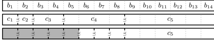
■ Figure 2 A lazy semi-sorted list. Top: Initial unsorted list of blocks b_1, \dots, b_{\mathcal{M}/B} . Middle: Initial chunks c_1 \preceq \dots \preceq c_5 . Bottom: The state after the first five blocks b_1, \dots, b_5 in the semi-sorted list have been accessed, i.e., the chunks c_1, \dots, c_4 have been made into semi-sorted sublists.
