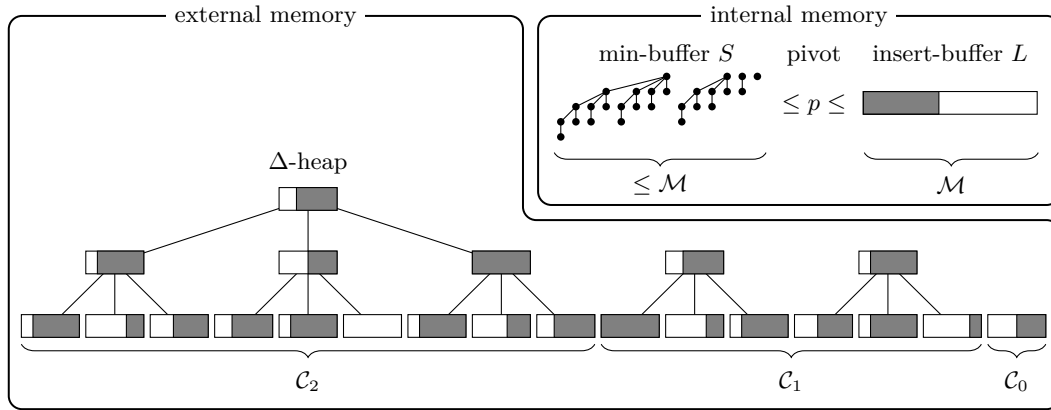
■ Figure 1 External-memory priority queue. All rectangles are buffers of capacity M , where the gray area illustrates elements in buffers.
