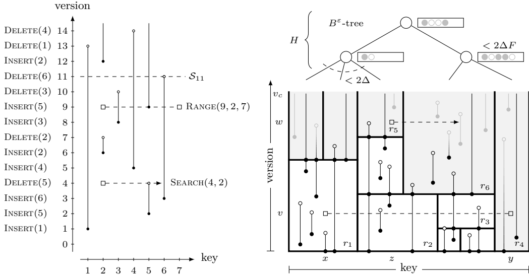
■ Figure 1 (Left) A list of updates performed on an initially empty set and the geometric interpretation of the updates. Vertical lines illustrate the half-open intervals of versions containing a key. Note that the key 3 is contained in versions [8, 10[ , i.e., versions 8 and 9, whereas the key 2 is contained in version 6 and versions [12, \infty[ . The topmost dashed line shows that version 11 of the set is S_{11} = \{1, 4, 5\} , the dashed line segment at version 9 shows that the result of the query \text{RANGE}(9, 2, 7) is \{3, 4, 5, 6\} , and the bottommost dashed arrow shows that the result of the successor search \text{SEARCH}(4, 2) is 6. (Right) A B^\epsilon -tree of the open rectangles and below the geometric interpretation of the updates, split into multiple rectangles, where gray rectangles are open rectangles. The black endpoints represent updates present in the rectangles and the gray endpoints represent buffered updates present in the buffers at the internal nodes of the B^\epsilon -tree. A query \text{RANGE}(v, x, y) is represented as the dashed line between two square endpoints, spanning rectangles r_1, r_2, r_3 , and r_4 , and a successor query \text{SEARCH}(w, z) is represented as the dashed arrow from a square endpoint, spanning two rectangles r_5 and r_6 . Black dots on vertical segments correspond to the upper endpoint of the segment in the rectangle below and the lower endpoint of the segment in the rectangle above.
