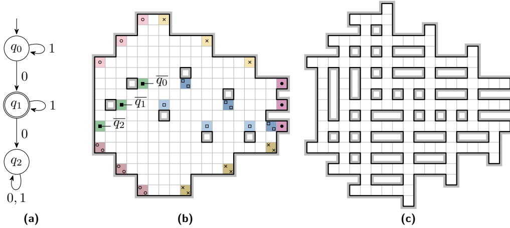
■ Figure 7 (a) The binary automaton A_0 that accepts all words containing exactly one 0. (b) The polyomino P(A_0) . Colors and symbols indicate congruence classes of pixels reachable from representatives \bar{q}_i . (c) P(A_0) turned into a maze M(A_0) by adding holes and pixels of degree 1.
