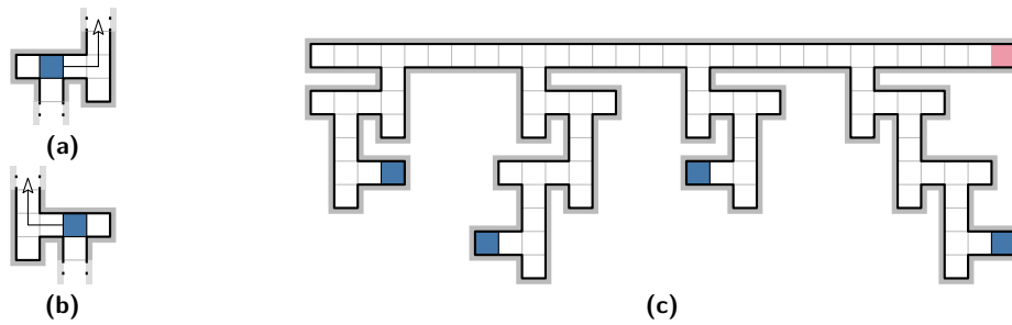
■ Figure 8 (a) 0-gadget, move sequence RU. (b) 1-gadget, move sequence LU. (c) The gathering instance for the words 10, 001, 01, and 111. A shortest supersequence is 10011 and the corresponding shortest gathering sequence is LU RU RU LU LU R. The particles gather in the red pixel.
