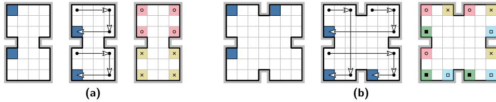
Figure 1 Two examples where gathering a set of particles is impossible in the full tilt model. Both examples depict, from left to right, a set of particles (blue squares) inside a polyomino, a sequence of moves leading to all possible configurations, and a partition of reachable positions yielding a congruence. Example (a) prohibits gathering by keeping the particles in different congruence classes, whereas the particles in (b) always occupy distinct positions of the same class.
