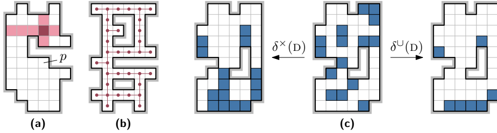
Figure 2 (a) A simple polyomino with a darkly shaded pixel at the intersection of two lightly shaded segments and a corner pixel p . (b) A non-simple maze and its dual graph. (c) Downwards moves in the blocking and merging variants of the full tilt model acting on a configuration.
