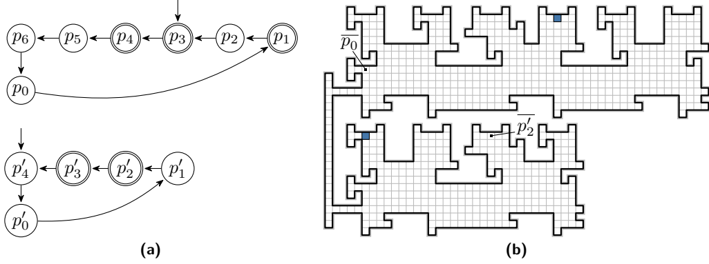
■ Figure 10 Instance of SUBSETGATHERING produced by the reduction from tally automata intersection. (a) Two tally automata, A_1, A_2 ; both accept the word of length 8. (b) The simple polyomino P(A_1, A_2) ; (RDLU)^8 LDRDL is a gathering sequence for its initial configuration C_0 .
