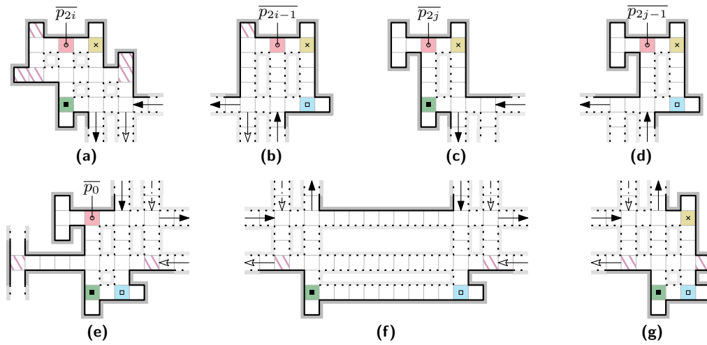
Figure 9 Gadgets used in the reduction from tally automata intersection. Pixels marked with colors and symbols indicate the cycle RDLU between pixels representing states, which is continued between gadgets via the black arrows. The stroked tiling pattern highlights pixels with a safe path to the goal area using the white arrows. Dotted areas specify optional holes that turn the simple polyomino into a maze. (a) Accepting state with even index. (b) Accepting state with odd index. (c) Rejecting state with even index. (d) Rejecting state with odd index. (e) Start gadget including \bar{p}_0 and access to the goal area to the left. (f) Bridge gadget. (g) End gadget connecting \bar{p}_0 to \bar{p}_1 .
