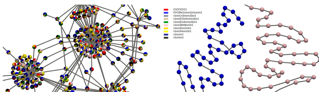
Figure 10 Partial views of mapper graphs derived from latent representations of the pre-trained (left) and fine-tuned (right) GraphMAE models. Fine-tuning refines and restructures the latent space, revealing its evolution during training. Both graphs are computed with 500 intervals, 40% overlap, and DBSCAN parameters \epsilon = 5 and \text{minPts} = 5 .
