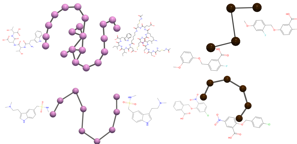
Figure 6 Four chain-like connected components with representative molecules identified by Chemical Mapper on the pre-trained GEM model. The components on the left are extracted from region 1 in Figure 5 (right), while the components on the right correspond to regions 9 (top) and 7 (bottom), respectively.
