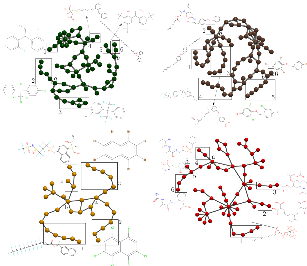
Figure 7 Four connected components with prominent branching structures identified by Chemical Mapper on the GEM model. The components are extracted from region 5 (top-left), region 8 (right), region 4 (bottom-left), and region 2 (bottom-right) in Figure 5 (right). Branches are highlighted using numbered boxes, and representative molecules are displayed adjacent to their corresponding branches or indicated with arrows.
