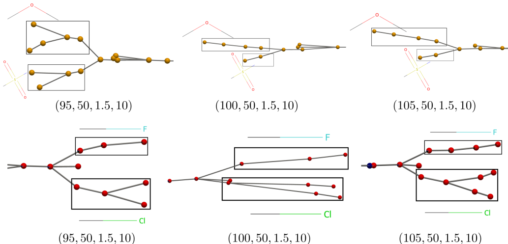
Figure 13 Two examples of local branches in mapper graphs generated under varying parameter settings (m, p, \epsilon, \text{minPts}) , where p , \epsilon , and \text{minPts} are fixed and m varies from 95 to 105. In both top and bottom cases, a component with the same branching structure and the same set of molecules persists across different m values, illustrating the stability of the mapper construction.
