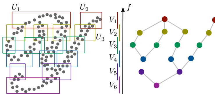
Figure 1 A simple illustration of mapper graph construction. Left: a point cloud X is equipped with a height function f . Middle: a cover \mathcal{U} = \{U_1, U_2, \dots\} of X is induced by a cover \mathcal{V} = \{V_1, V_2, \dots\} of f(X) consisting of 6 intervals with 25% overlap. Right: the 1D nerve of \mathcal{U} yields the mapper graph.
