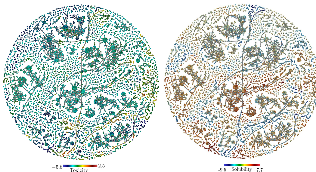
Figure 9 Mapper graphs of molecular representations from the pre-trained GEM model, computed using the same experimental settings as in Figure 5. Nodes are colored according to molecular toxicity (left) and solubility (right), as discussed in Section 3.2.3 and Section 2.
