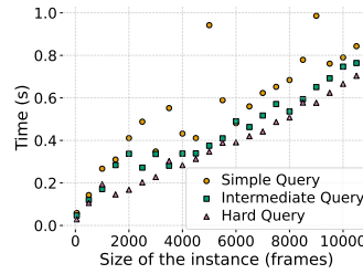
■ Figure 6 Execution times Bigger instance sizes.
