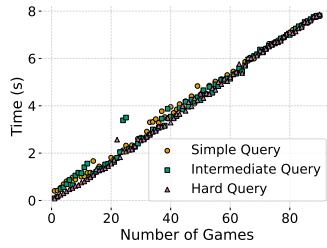
■ Figure 5 Execution times Games are gradually added.
