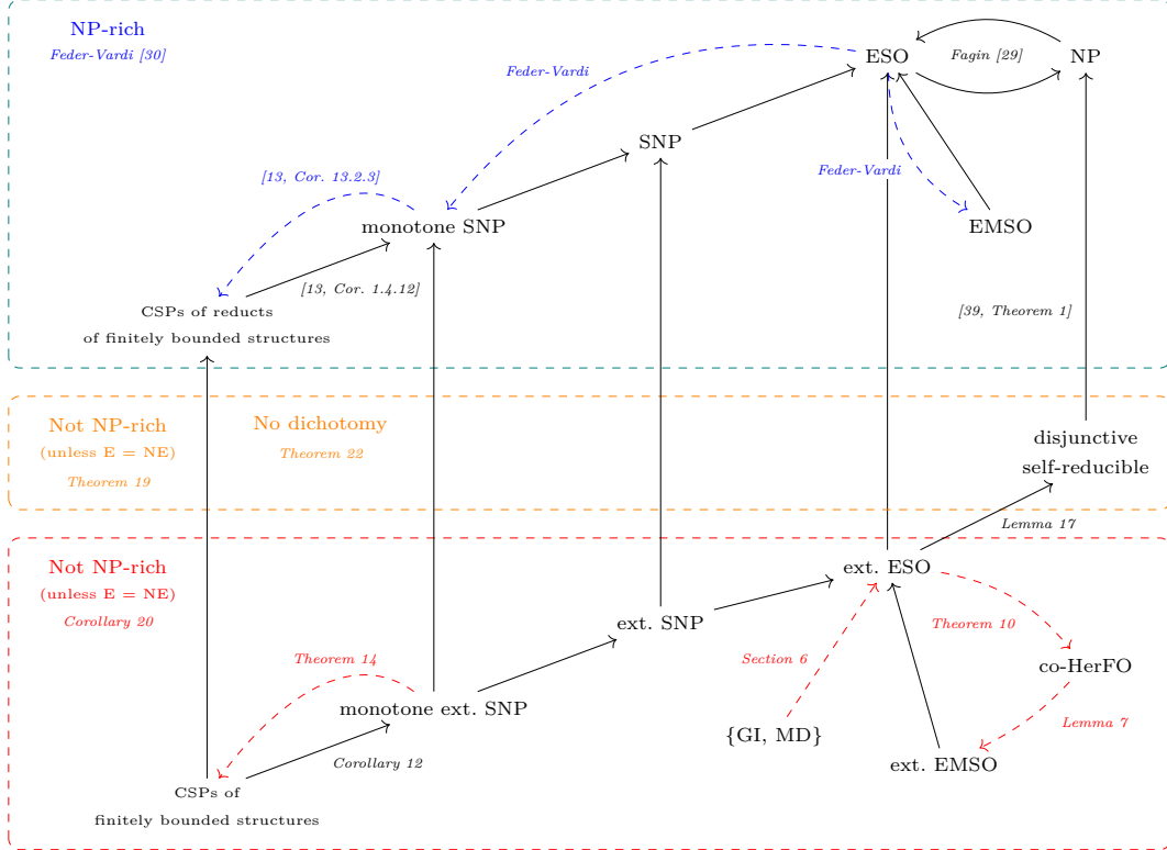
■ Figure 1 Classes of computational problems studied in this paper. Solid arcs indicate inclusions, and a dashed arc from A to B indicates that every problem in A is polynomial-time equivalent to a problem in B – for a cleaner picture we omit the solid arc from extensional EMSO to EMSO. GI stands for the Graph Isomorphism problem, and MD for the Monotone Dualization problem.
