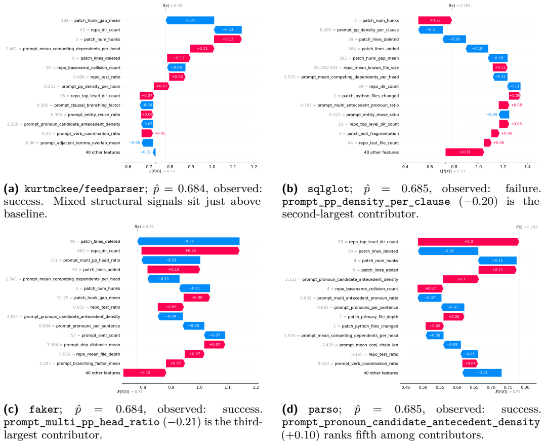
■ Figure 6 SHAP waterfalls for four representative average-difficulty tasks ( \hat{p} \approx 0.68 , E[f(x)] = 0.73 , XGBoost, any_success ). In three of four cases a prompt feature ranks among the top contributors, with magnitudes comparable to the structural features for those tasks.
