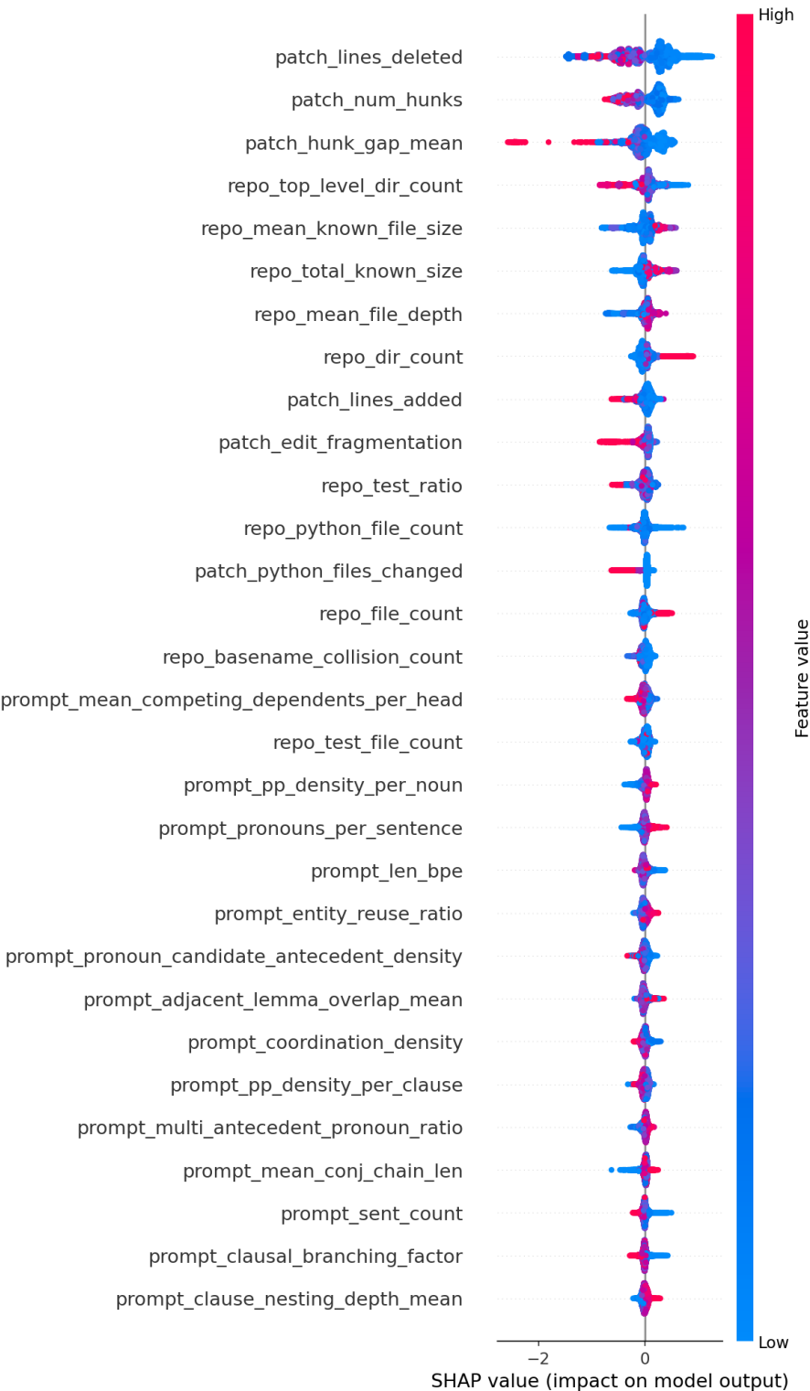
Figure 4 SHAP summary plot for any_success.
