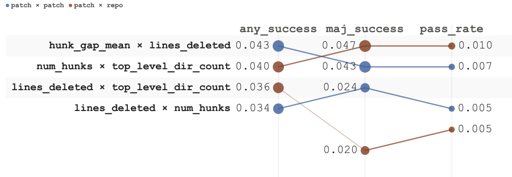
■ Figure 2 Rank-magnitude bump chart for the top four SHAP interaction pairs by mean absolute interaction value averaged across outcome targets.
