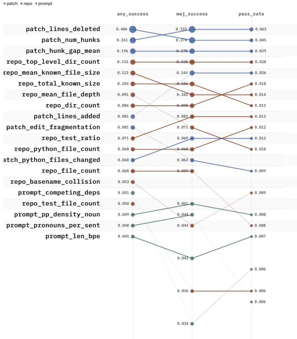
Figure 3 Rank-magnitude bump chart for the top 20 features by mean absolute SHAP value across three outcome targets (XGBoost, held-out test set). Each dot is one feature–outcome pair; dot area is proportional to mean absolute SHAP. Connecting lines trace rank shifts across outcomes; steep slopes indicate instability. Color encodes feature family: patch (blue), repo (red-brown), prompt (green). The top six ranks are stable across all three outcomes (near-flat lines); prompt features first appear at rank 16 with visibly smaller dots and show greater rank instability below rank 16.
