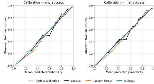
■ Figure 1 Calibration reliability diagrams.
