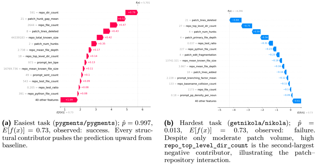
■ Figure 5 SHAP waterfalls for extreme-difficulty tasks (XGBoost, any_success target). All values in log-odds space; E[f(x)] = 0.73 for both.
