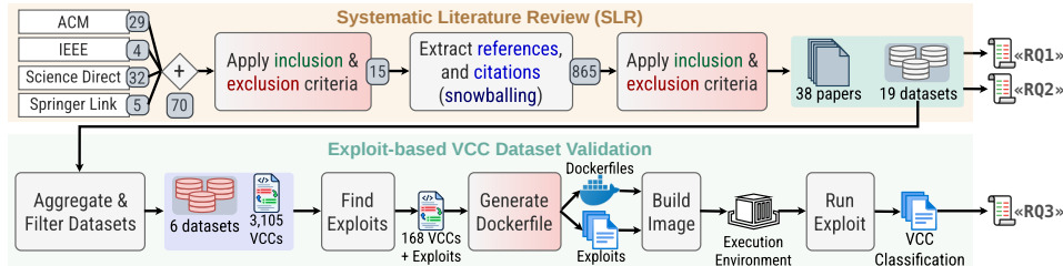
■ Figure 1 Overview of our two-part study. Part 1: the literature review to answer RQ1 and RQ2. Part 2: the exploit-based validation, aggregating 6 datasets into 3,105 samples, screening to the 168 with documented exploits, and testing each labeled commit and its parent to answer RQ3.
