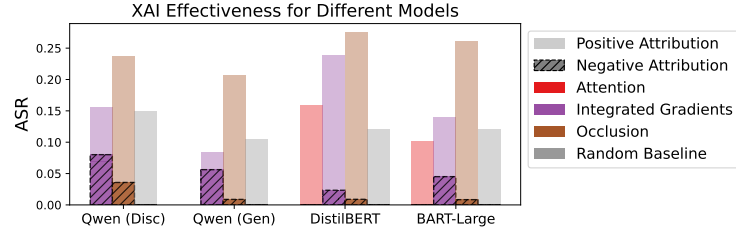
■ Figure 1 Effectiveness of different XAI explainers in guiding Metamorphic Ablation.
