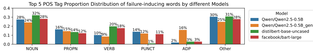
■ Figure 3 POS analysis of failure-inducing words.
