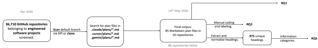
■ Figure 1 Process for identifying Agent Plan Markdown files in GitHub repositories.
