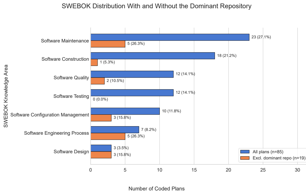
■ Figure 2 Distribution of Agent Plans across SWEBOK knowledge areas.
