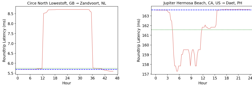
■ Figure 10 Left: Estimates on cable Circe North calculated over 48 hours. Estimators ( \hat{r}_{SL} , \hat{r}_{SLu} ) given by (green/top, blue/bottom) horizontal lines and \Delta_P in red. Right: Estimates on cable Jupiter calculated over 24 hours. Estimators ( \hat{r}_{SL} , \hat{r}_{SLu} ) given by (green/bottom, blue/top) horizontal lines and \Delta_P in red. Since there are no underlying LSes in R1 , R2 (not shown), we expect \hat{r}_{SLu} to be superior as \hat{r}_{SL} is impacted by the unusually persistent congestion over most of the period.
