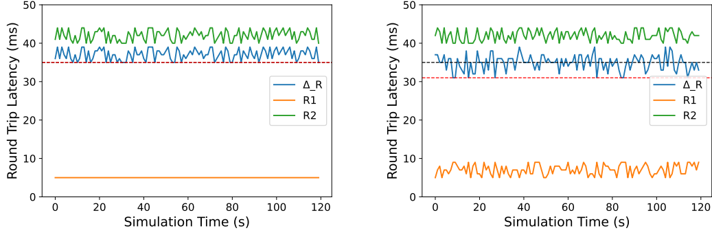
■ Figure 7 An illustration of how bidirectional noise corrupts a minimum estimate taken by \hat{r}_n := \min_j(\underline{r}_{2j} - \underline{r}_{1j}) , using artificial data. Let R1 and R2 have underlying minimum delay values of 5ms and 40ms respectively. The true minimum RTT for \Delta_R is thus 35ms and is indicated by the black dashed line in each plot. The naive minimum estimate is indicated by the red dashed line. Left: \Delta_R latency when some random congestion term \varepsilon_j \in [0, 5] is added to \underline{r}_{2j} \in R2 such that \underline{r}_{2j}' = \underline{r}_{2j} + \varepsilon_j . Here, the naive estimator performs excellently as the noise is purely positive, which the minimum based definition can handle. However, as shown in Figure 5, such a congestion model does not represent real-world data. Right: We add an independent random congestion term \eta_j \in [0, 5] to R1 also such that \underline{r}_{1j}' = \underline{r}_{1j} + \eta_j . As this operates in the negative direction, the minimum-based definition of the naive estimator follows it (naively) below the true minimum whenever the negatively directed noise in R1 defeats the positive noise in R2 . We see that even when adding slight congestion to R1 the naive method underestimates the true minimum latency. In practice this underestimation can be very large even if only a single value of \eta_j is large.
