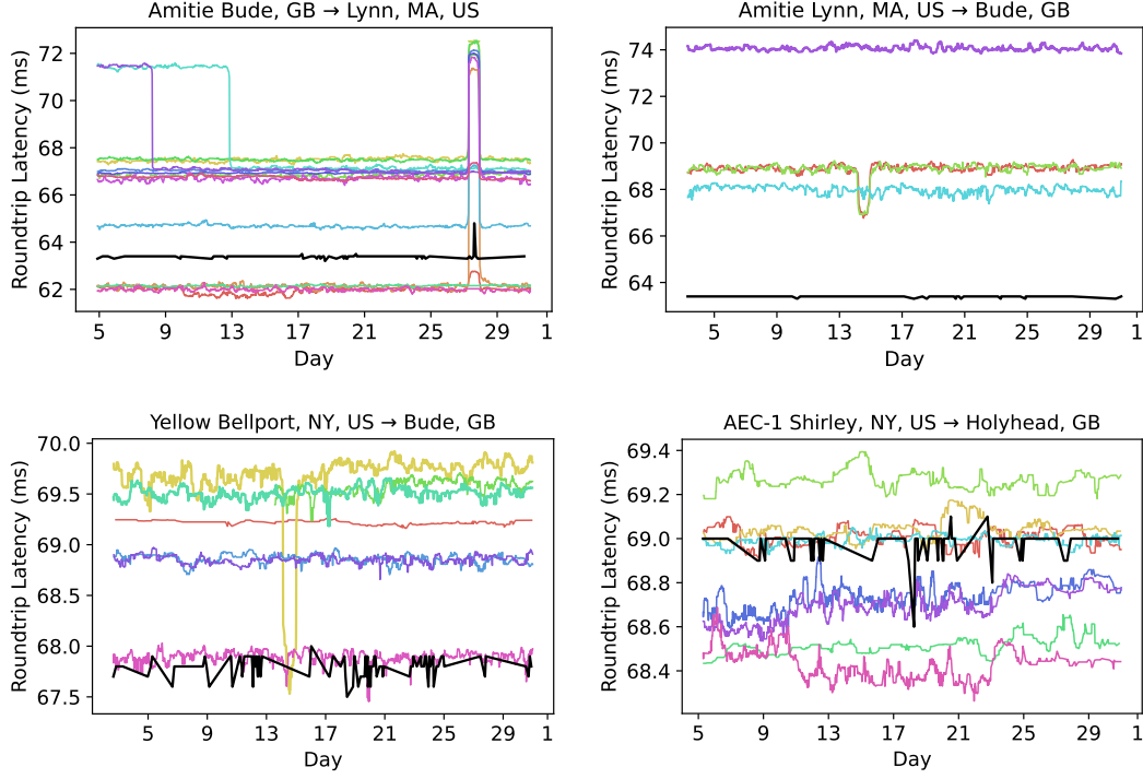
■ Figure 6 All available \Delta_P timeseries for four different SLs. In each case the distribution of levels has a different relationship to the ground truth \Delta_P [full black line].
