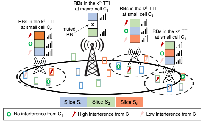
Figure 2 Typical multi-cell deployment with a macro-cell ( C_1 ) and small cells ( C_2 , C_3 , and C_4 ). The figure depicts how RBs at a given TTI are scheduled across users belonging to three different slices at each cell. Muting the transmission of an RB at a cell (say, the second RB at C_1 , as shown) ensures that users scheduled on that RB at neighboring cells do not experience interference from C_1 . The amount of interference from C_1 experienced by a user in a neighboring cell depends on the user's proximity to C_1 , and impacts that user's channel quality (illustrated by signal-strength bars).
