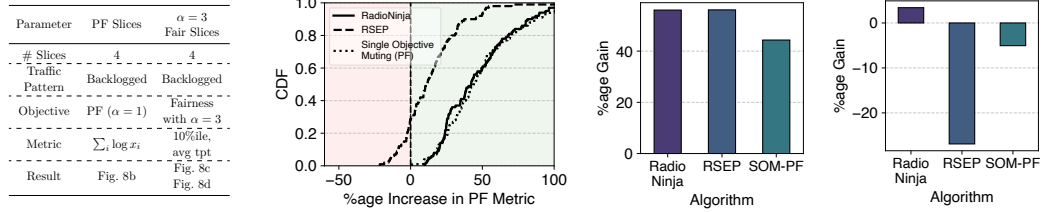
(d) % increase in avg throughput across users in \alpha = 3 Fair slices.
