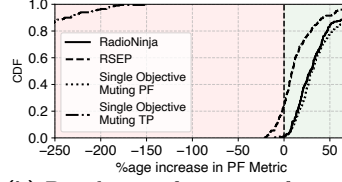
(b) Per slice performance of PF slices.
