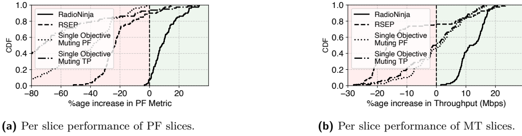
Figure 11 RadioNinja's, RSEP's and SOM-PF's and SOM-TP's impact on slice-level performance when compared to RadioSaber (no muting) for (a) PF slices and (b) Max TP slices under Scenario 1 (Table 7a) with unequal slice quotas and distribution across cells.
