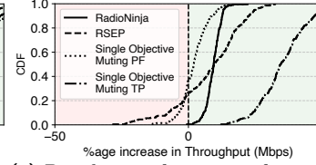
(c) Per slice performance of MT slices.
