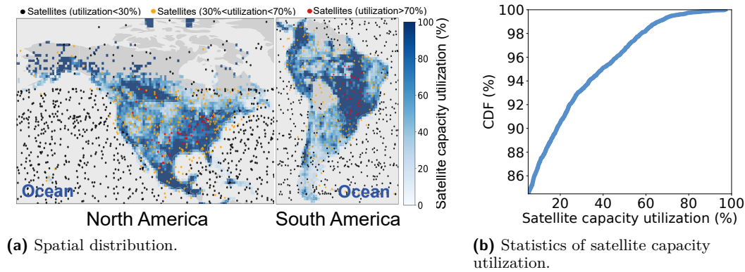
■ Figure 2 Underutilization of Starlink satellites based on Cloudflare [32].
