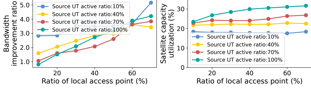
■ Figure 19 Impact of the scale of local access point UTs.
