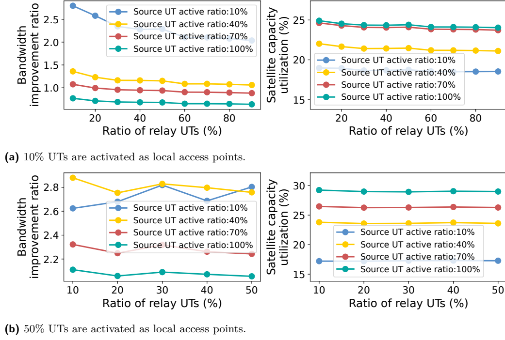
■ Figure 18 Impact of the scale of relay UTs.
