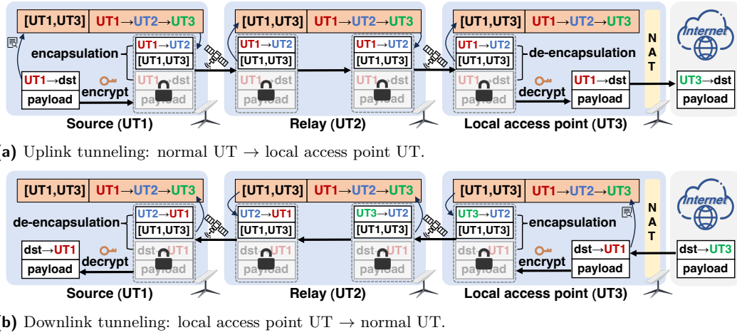
■ Figure 8 CrowdLink's transparent inter-UT traffic tunneling to satellites.
