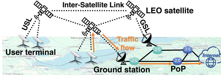
■ Figure 3 The state-of-the-art LEO satellite network architecture.
