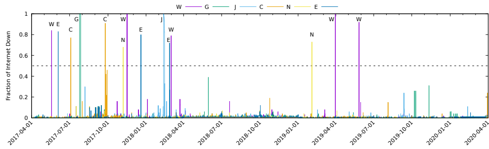
■ Figure 10 Islands detected across 3 years using six VPs. Datasets A28-A39.
