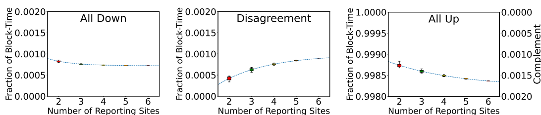
■ Figure 2 Distribution of block-time fraction: all-down (left), disagreement (center), and all-up (right), events \geq 1 hour. Data: 3.7M blocks, 2017-10-06 to -11-16, A30.
