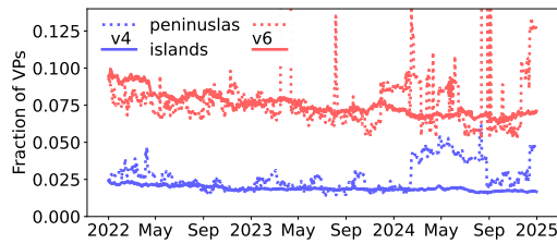
■ Figure 6 Fraction of VPs observing islands and peninsulas for IPv4 and IPv6, 2022–2025.
