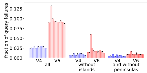
■ Figure 7 Atlas queries from all available VPs to 13 Root Servers for IPv4 and IPv6 on 2022-07-23.
