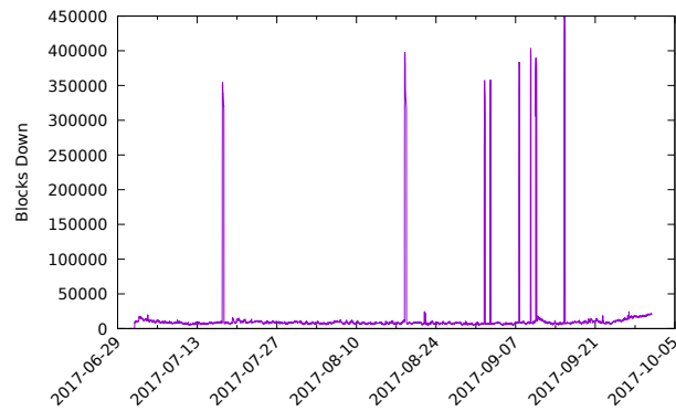
■ Figure 9 Unreachable blocks over time. Large spikes are unreachability to Chinese-allocated IPv4 addresses. Dataset: A29, 2017q3.
