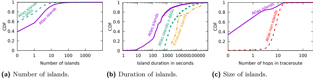
■ Figure 5 CDF of islands detected by Chiloe for data from Trinocular (3 years, Datasets A28-A39) and Atlas (2021q3).
