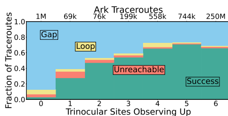
■ Figure 8 Ark traceroutes sent to targets under partial outages (2017-10-10 to -31). Dataset A30.
