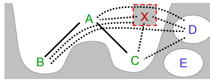
■ Figure 1 A , B and C are the connected core, B and C peninsulas, D and E islands, X is out.
