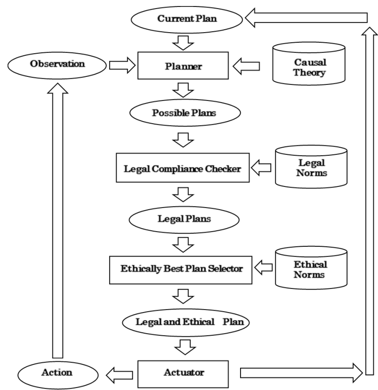
■ Figure 1 The architecture for RECOMP planning.
