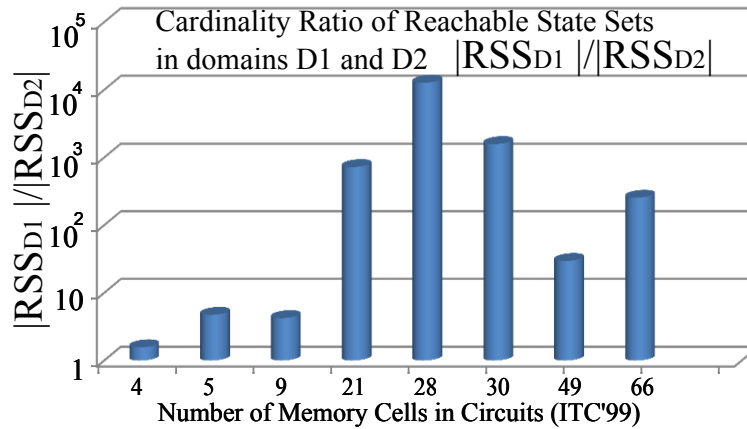
■ Figure 8 Logic Domain Comparison: Size Ratio of RSS.
