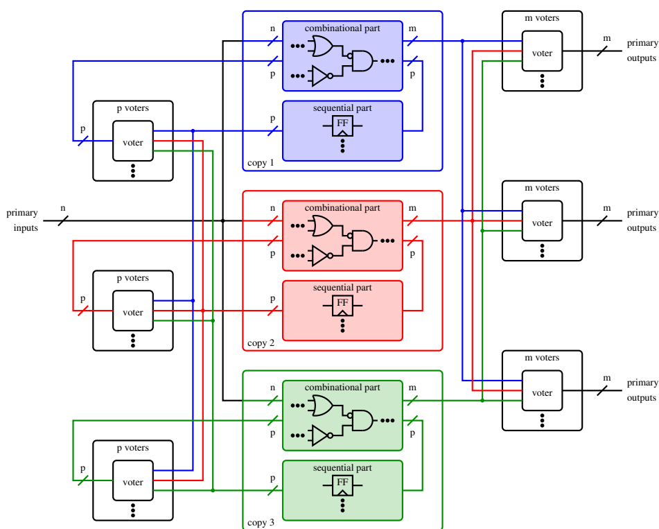
■ Figure 2 Full TMR with triplicated voters after the p internal FFs and the m primary outputs.
