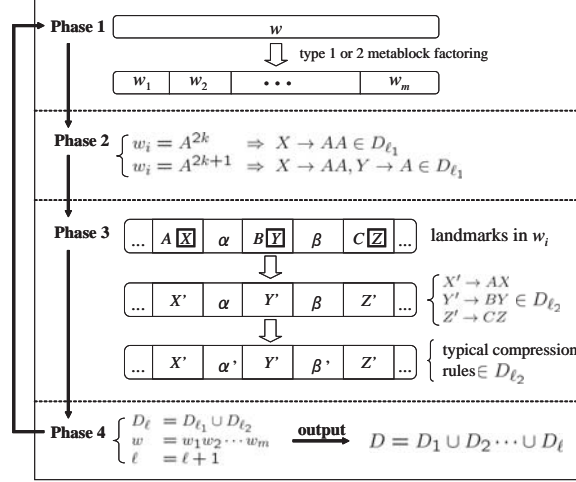
Figure 5: The flow of LCA* for a string w .
