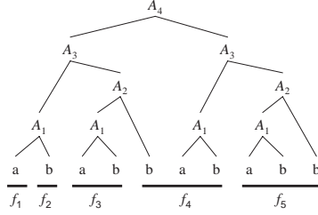
Figure 1: LZ-factorization and CFG derivation.
