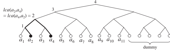
Figure 2: The alphabet tree for \Sigma \cup N = \{a_1, \dots, a_{11}\} .
